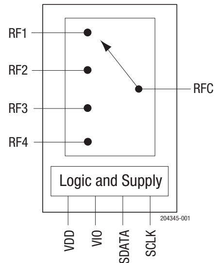
Figure 1. SKY19249-686LF Block Diagram
