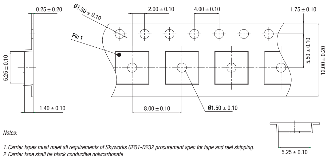
Figure 24. SKY66297-11 Tape and Reel Dimensions
