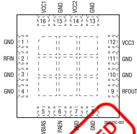
Figure 2. SKY66297-11 Pinout (Top View)
