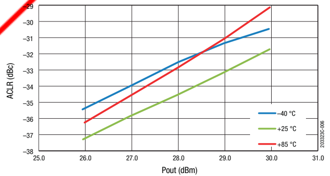
Figure 6. ACLR vs Pout Across Temperature (20 MHz LTE, 8.5 dB PAR Signal)
