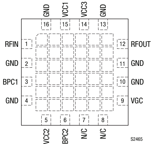
Figure 2. SKY65370-11 Pinout (Top View)
