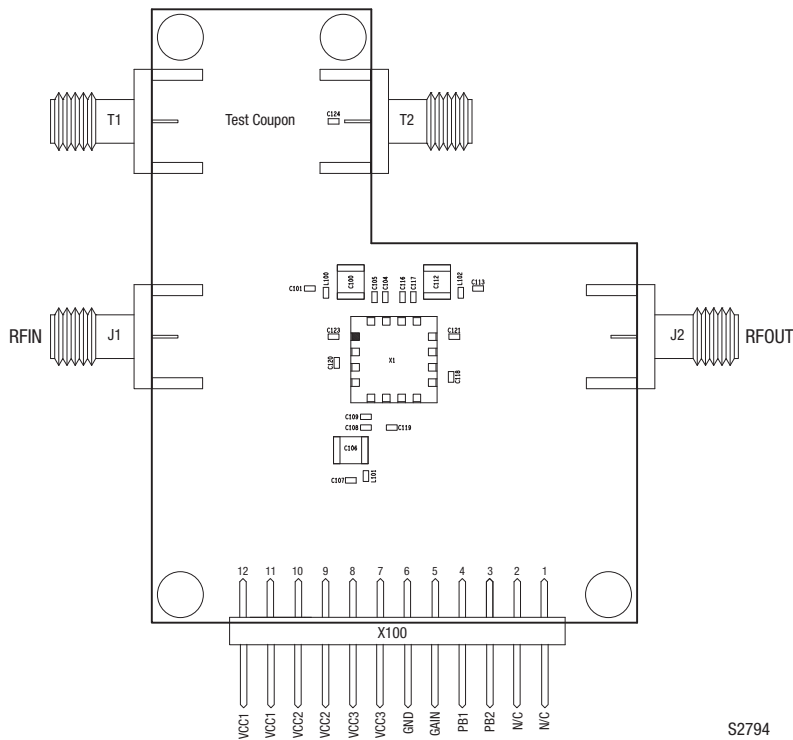
Figure 3. SKY65370-11 Evaluation Board Assembly Diagram
